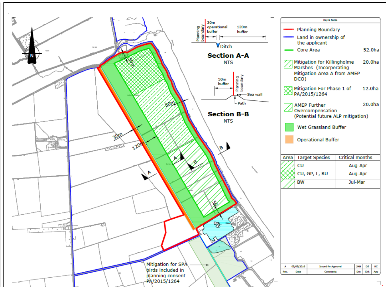
Figure 1.3 – General Layout of HMWG
